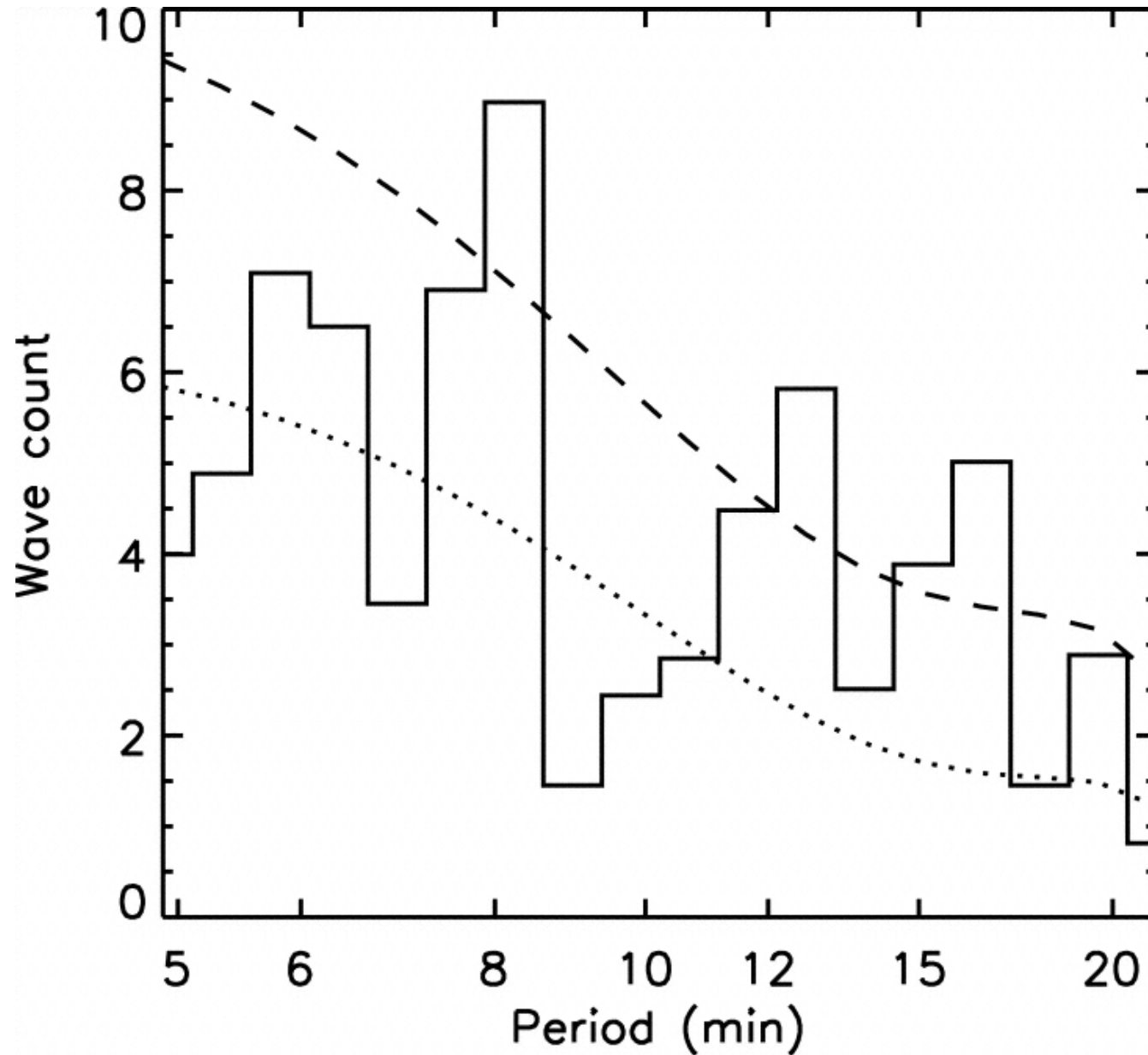
Fig. 6. from Hydrogen Ly Intensity Oscillations Observed by the Solar and Heliospheric Observatory Ultraviolet Coronagraph Spectrometer Morgan, Habbal, & Li 2004 ApJ 605 521 doi:10.1086/382203 https://dx.doi.org/10.1086/382203 © 2004. The American Astronomical Society. All rights reserved. Printed in U.S.A.
