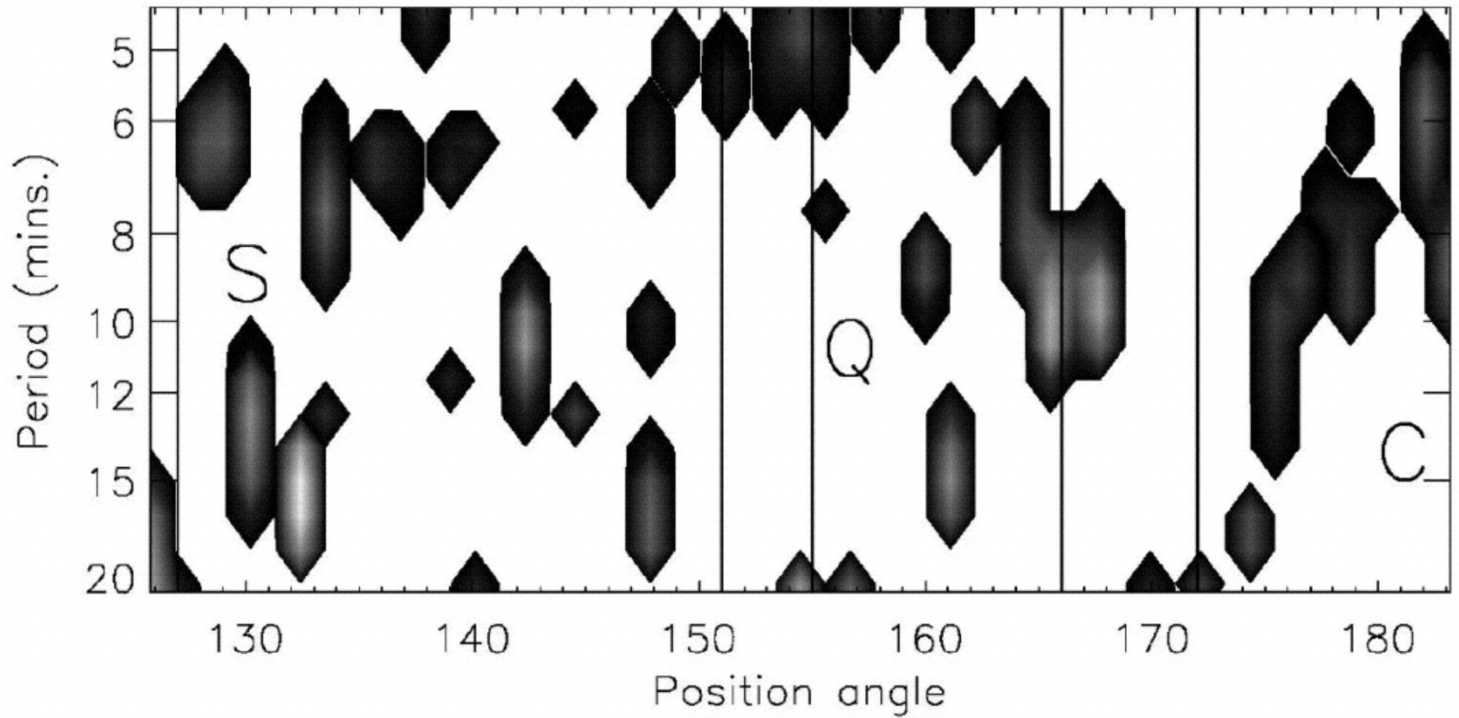
Fig. 5. from Hydrogen Ly Intensity Oscillations Observed by the Solar and Heliospheric Observatory Ultraviolet Coronagraph Spectrometer Morgan, Habbal, & Li 2004 ApJ 605 521 doi:10.1086/382203 https://dx.doi.org/10.1086/382203 © 2004. The American Astronomical Society. All rights reserved. Printed in U.S.A.
