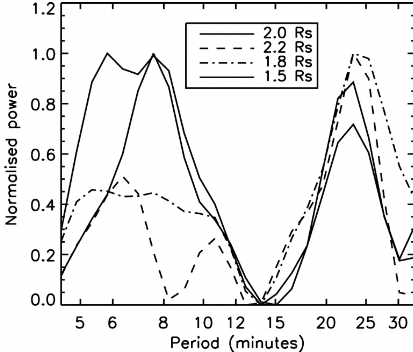
Fig. 4. from Hydrogen Ly Intensity Oscillations Observed by the Solar and Heliospheric Observatory Ultraviolet Coronagraph Spectrometer Morgan, Habbal, & Li 2004 ApJ 605 521 doi:10.1086/382203 https://dx.doi.org/10.1086/382203 © 2004. The American Astronomical Society. All rights reserved. Printed in U.S.A.
