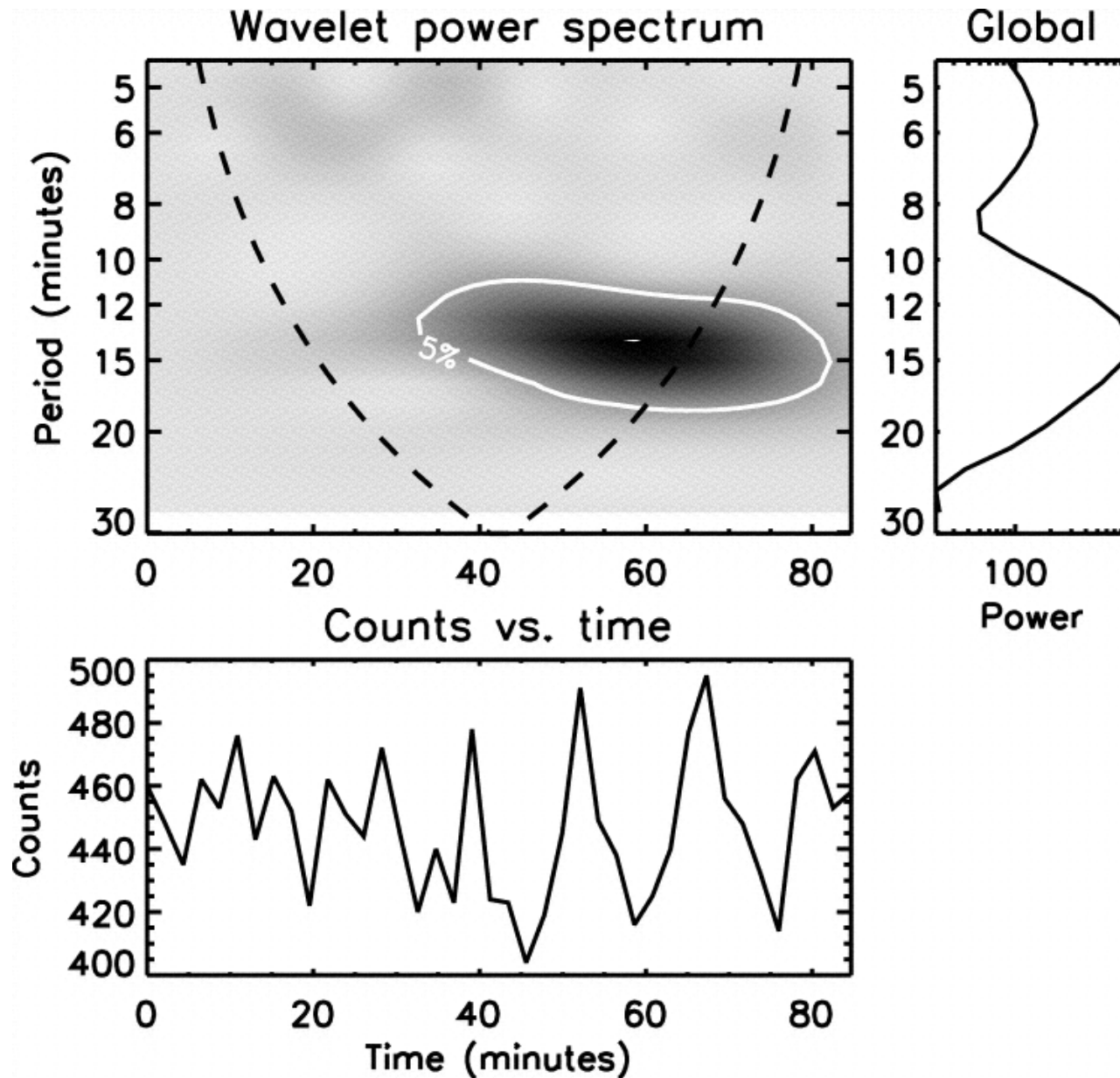
Fig. 3. from Hydrogen Ly Intensity Oscillations Observed by the Solar and Heliospheric Observatory Ultraviolet Coronagraph Spectrometer Morgan, Habbal, & Li 2004 ApJ 605 521 doi:10.1086/382203 https://dx.doi.org/10.1086/382203
