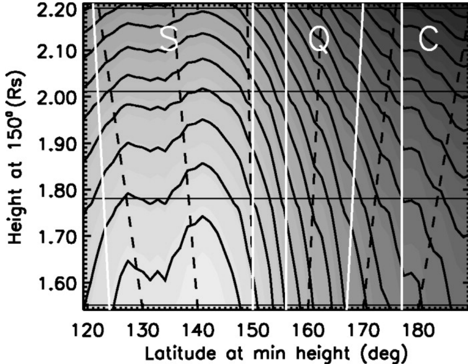
Fig. 1. from Hydrogen Ly Intensity Oscillations Observed by the Solar and Heliospheric Observatory Ultraviolet Coronagraph Spectrometer Morgan, Habbal, & Li 2004 ApJ 605 521 doi:10.1086/382203 https://dx.doi.org/10.1086/382203 © 2004. The American Astronomical Society. All rights reserved. Printed in U.S.A.
