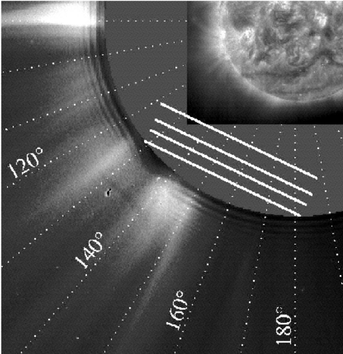
Fig. 1. from Hydrogen Ly Intensity Oscillations Observed by the Solar and Heliospheric Observatory Ultraviolet Coronagraph Spectrometer Morgan, Habbal, & Li 2004 ApJ 605 521 doi:10.1086/382203 https://dx.doi.org/10.1086/382203 © 2004. The American Astronomical Society. All rights reserved. Printed in U.S.A.
