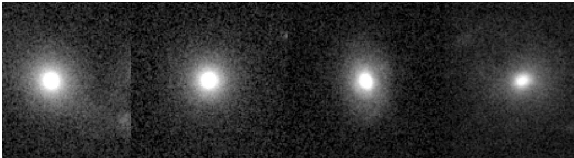
Fig. 1. from The Fundamental Plane of Field EarlyType Galaxies at z = 1 van der Wel et al. 2004 ApJL 601 L5 doi:10.1086/381887 https://dx.doi.org/10.1086/381887 © 2004. The American Astronomical Society. All rights reserved. Printed in U.S.A.
