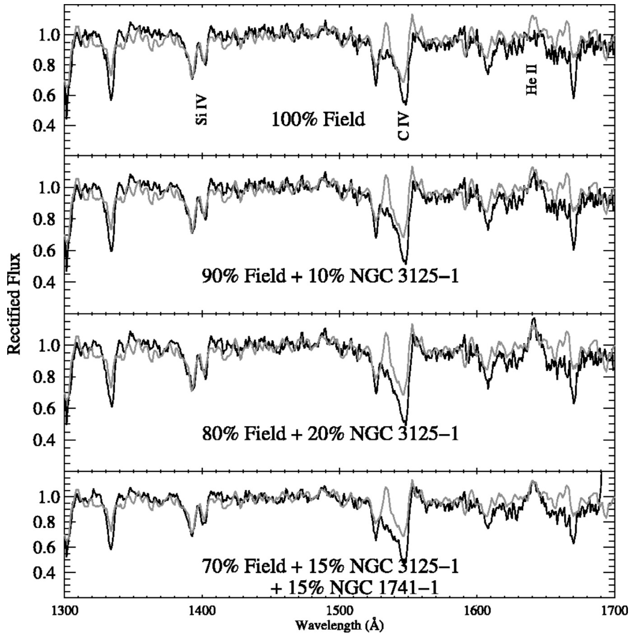
Fig. 3. from NGC 31251: The Most Extreme WolfRayet Star Cluster Known in the Local Universe Chandar, Leitherer, & Tremonti 2004 ApJ 604 153 doi:10.1086/381723 https://dx.doi.org/10.1086/381723 © 2004. The American Astronomical Society. All rights reserved. Printed in U.S.A.
