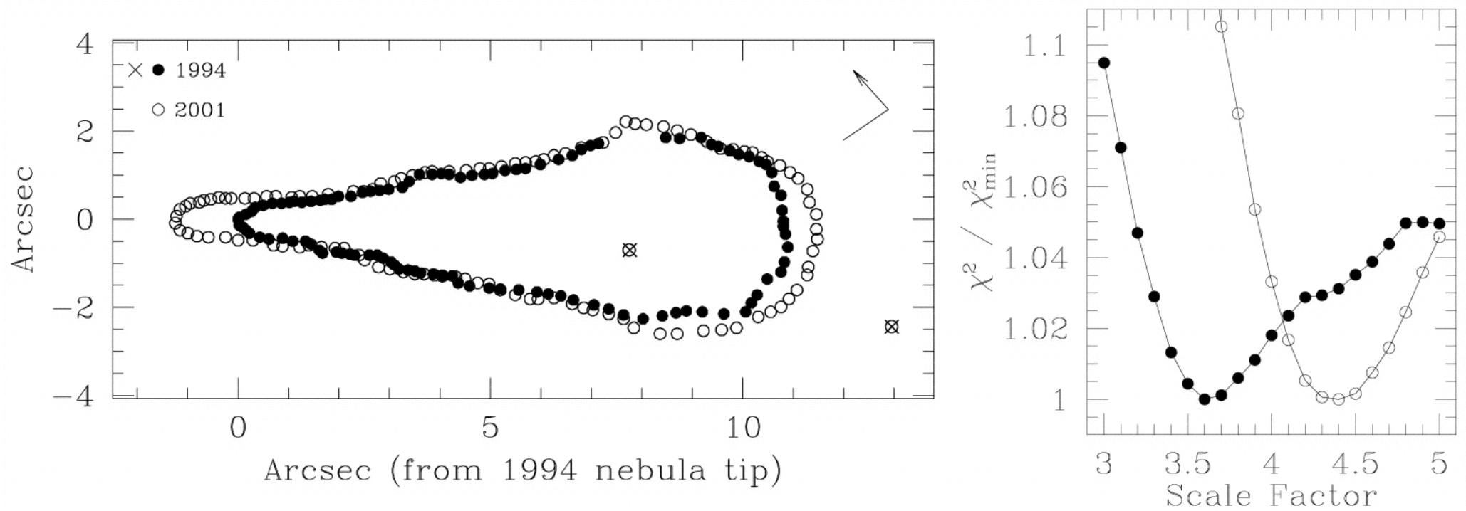
Fig. 2. from Smashing the Guitar: An Evolving Neutron Star Bow Shock Chatterjee & Cordes 2004 ApJL 600 L51 doi:10.1086/381498 https://dx.doi.org/10.1086/381498 © 2004. The American Astronomical Society. All rights reserved. Printed in U.S.A.
