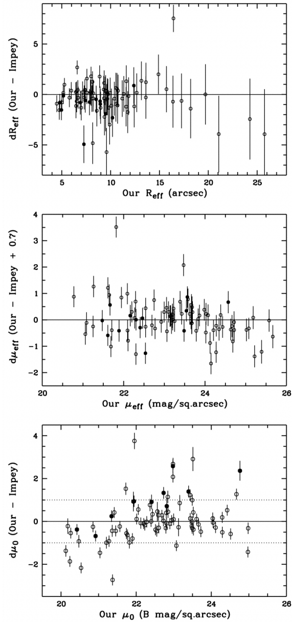
Fig. 9. from Low Surface Brightness Galaxies in the Sloan Digital Sky Survey. I. Search Method and Test Sample Kniazev et al. 2004 AJ 127 704 doi:10.1086/381061 https://dx.doi.org/10.1086/381061
