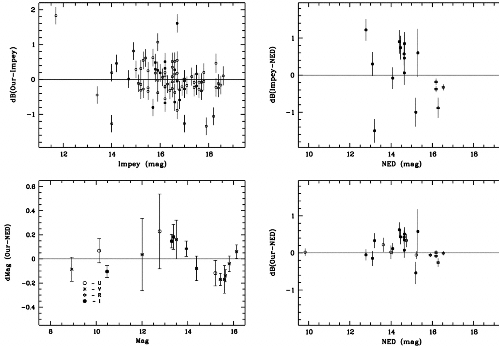
Fig. 8. from Low Surface Brightness Galaxies in the Sloan Digital Sky Survey. I. Search Method and Test Sample Kniazev et al. 2004 AJ 127 704 doi:10.1086/381061 https://dx.doi.org/10.1086/381061 © 2004. The American Astronomical Society. All rights reserved. Printed in U.S.A.
