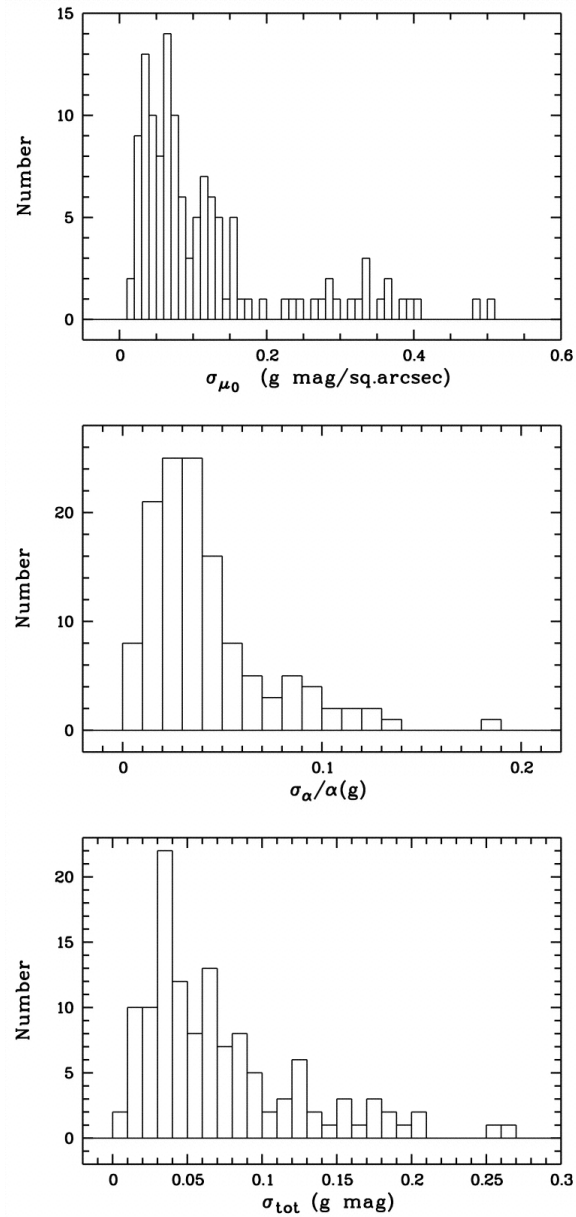
Fig. 6. from Low Surface Brightness Galaxies in the Sloan Digital Sky Survey. I. Search Method and Test Sample Kniazev et al. 2004 AJ 127 704 doi:10.1086/381061 https://dx.doi.org/10.1086/381061
