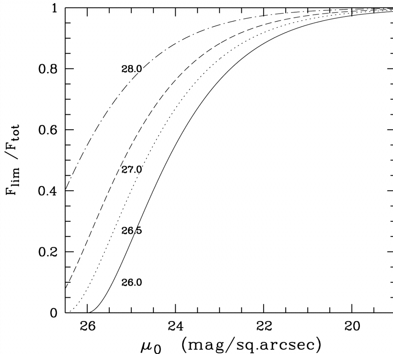
Fig. 5. from Low Surface Brightness Galaxies in the Sloan Digital Sky Survey. I. Search Method and Test Sample Kniazev et al. 2004 AJ 127 704 doi:10.1086/381061 https://dx.doi.org/10.1086/381061 © 2004. The American Astronomical Society. All rights reserved. Printed in U.S.A.
