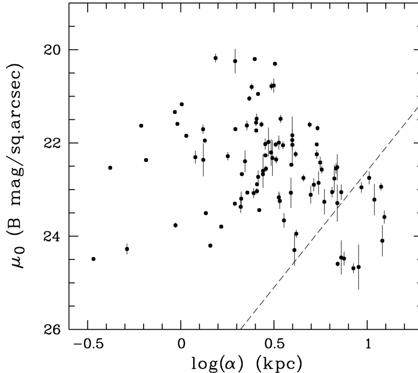
Fig. 16. from Low Surface Brightness Galaxies in the Sloan Digital Sky Survey. I. Search Method and Test Sample Kniazev et al. 2004 AJ 127 704 doi:10.1086/381061 https://dx.doi.org/10.1086/381061 © 2004. The American Astronomical Society. All rights reserved. Printed in U.S.A.
