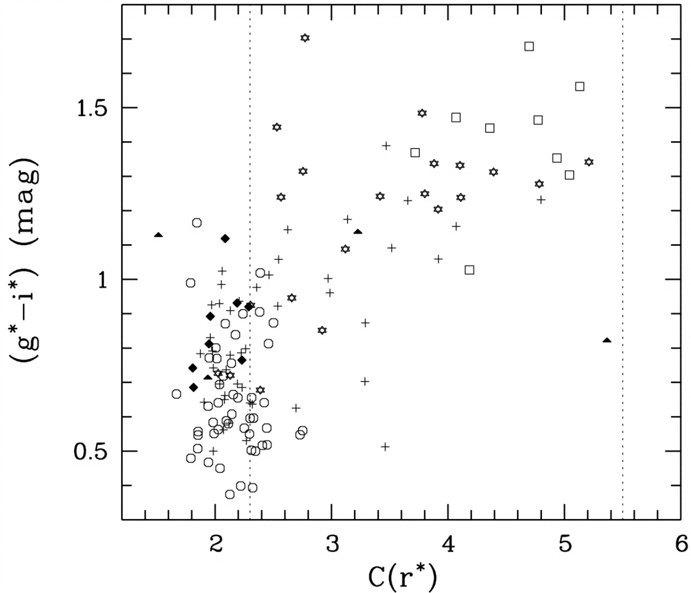
Fig. 14. from Low Surface Brightness Galaxies in the Sloan Digital Sky Survey. I. Search Method and Test Sample Kniazev et al. 2004 AJ 127 704 doi:10.1086/381061 https://dx.doi.org/10.1086/381061 © 2004. The American Astronomical Society. All rights reserved. Printed in U.S.A.
