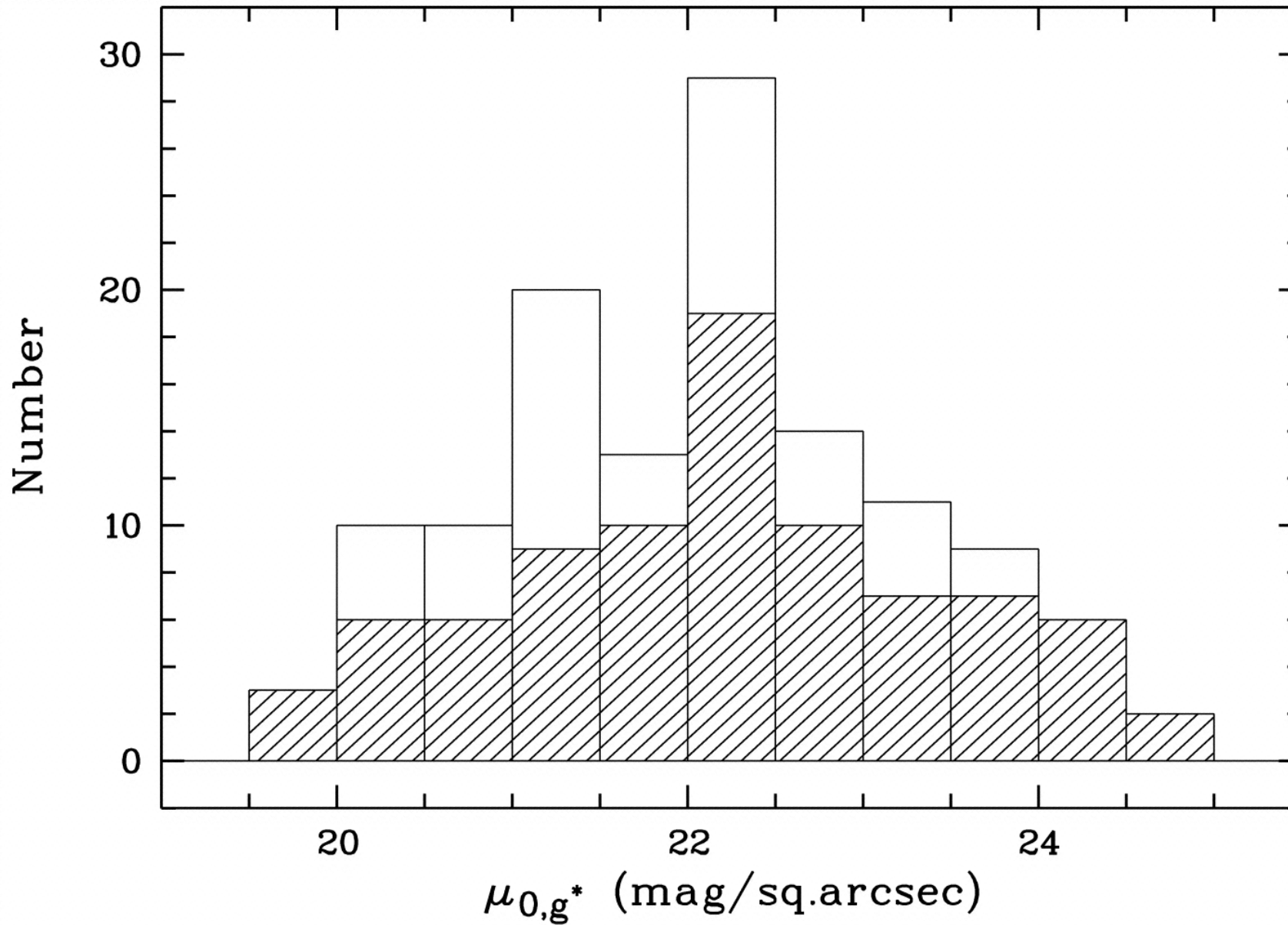
Fig. 11. from Low Surface Brightness Galaxies in the Sloan Digital Sky Survey. I. Search Method and Test Sample Kniazev et al. 2004 AJ 127 704 doi:10.1086/381061 https://dx.doi.org/10.1086/381061 © 2004. The American Astronomical Society. All rights reserved. Printed in U.S.A.
