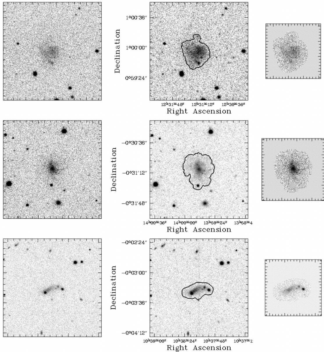
Fig. 1. from Low Surface Brightness Galaxies in the Sloan Digital Sky Survey. I. Search Method and Test Sample Kniazev et al. 2004 AJ 127 704 doi:10.1086/381061 https://dx.doi.org/10.1086/381061
