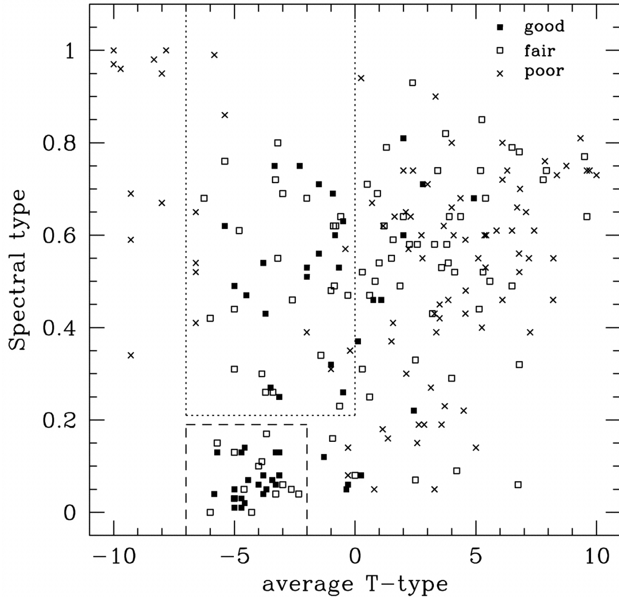
Fig. 9. from The Evolution of EarlyType Field Galaxies Selected from a NICMOS Map of the Hubble Deep Field North Stanford et al. 2004 AJ 127 131 doi:10.1086/380612 https://dx.doi.org/10.1086/380612 © 2004. The American Astronomical Society. All rights reserved. Printed in U.S.A.
