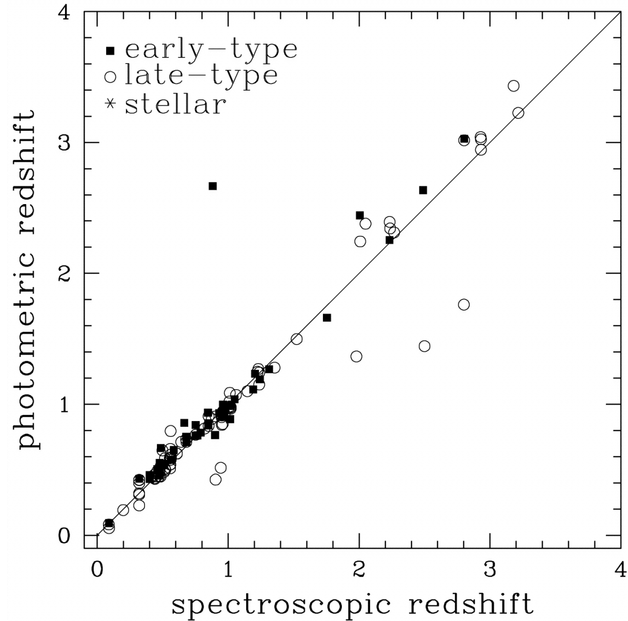
Fig. 8. from The Evolution of EarlyType Field Galaxies Selected from a NICMOS Map of the Hubble Deep Field North Stanford et al. 2004 AJ 127 131 doi:10.1086/380612 https://dx.doi.org/10.1086/380612 © 2004. The American Astronomical Society. All rights reserved. Printed in U.S.A.
