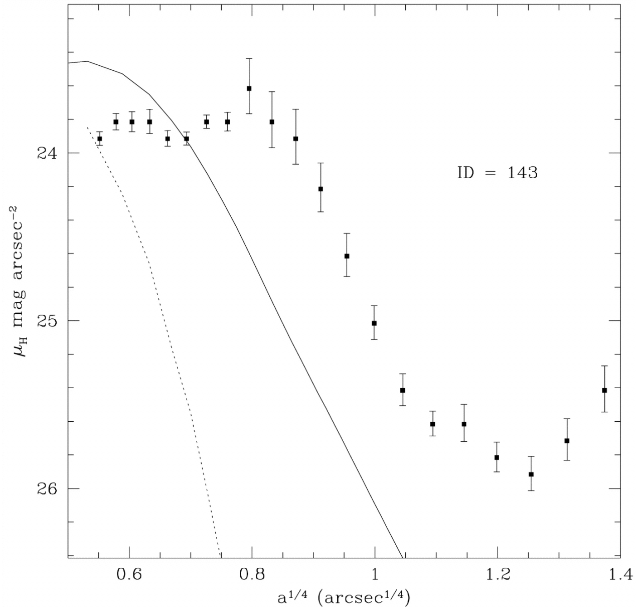
Fig. 7. from The Evolution of EarlyType Field Galaxies Selected from a NICMOS Map of the Hubble Deep Field North Stanford et al. 2004 AJ 127 131 doi:10.1086/380612 https://dx.doi.org/10.1086/380612 © 2004. The American Astronomical Society. All rights reserved. Printed in U.S.A.
