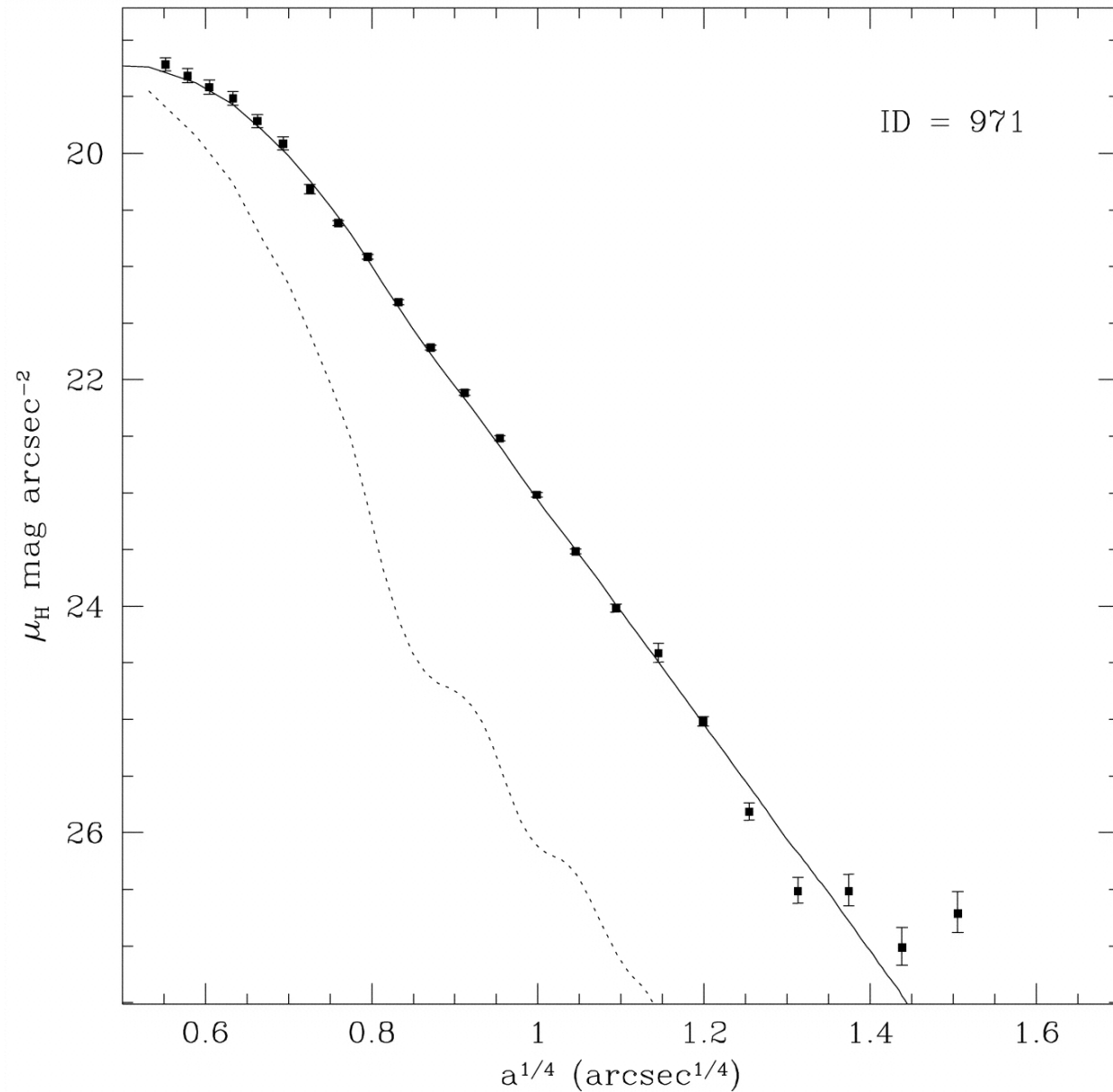
Fig. 7. from The Evolution of EarlyType Field Galaxies Selected from a NICMOS Map of the Hubble Deep Field North Stanford et al. 2004 AJ 127 131 doi:10.1086/380612 https://dx.doi.org/10.1086/380612 © 2004. The American Astronomical Society. All rights reserved. Printed in U.S.A.
