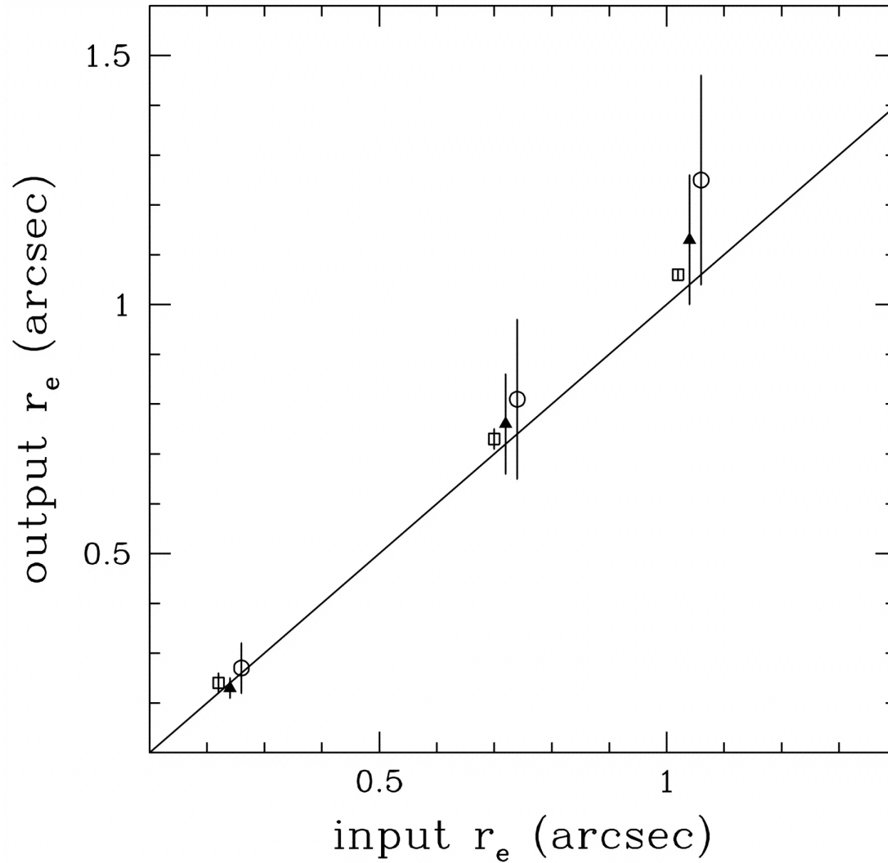
Fig. 6. from The Evolution of EarlyType Field Galaxies Selected from a NICMOS Map of the Hubble Deep Field North Stanford et al. 2004 AJ 127 131 doi:10.1086/380612 https://dx.doi.org/10.1086/380612 © 2004. The American Astronomical Society. All rights reserved. Printed in U.S.A.
