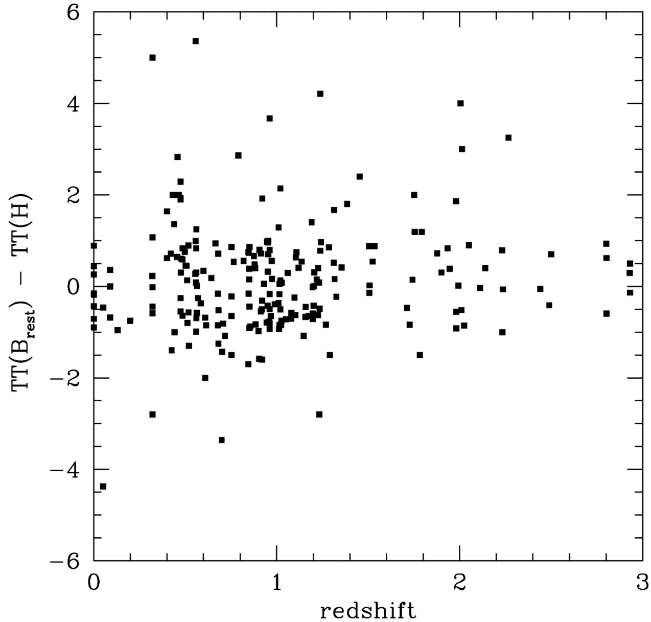
Fig. 3. from The Evolution of EarlyType Field Galaxies Selected from a NICMOS Map of the Hubble Deep Field North Stanford et al. 2004 AJ 127 131 doi:10.1086/380612 https://dx.doi.org/10.1086/380612 © 2004. The American Astronomical Society. All rights reserved. Printed in U.S.A.
