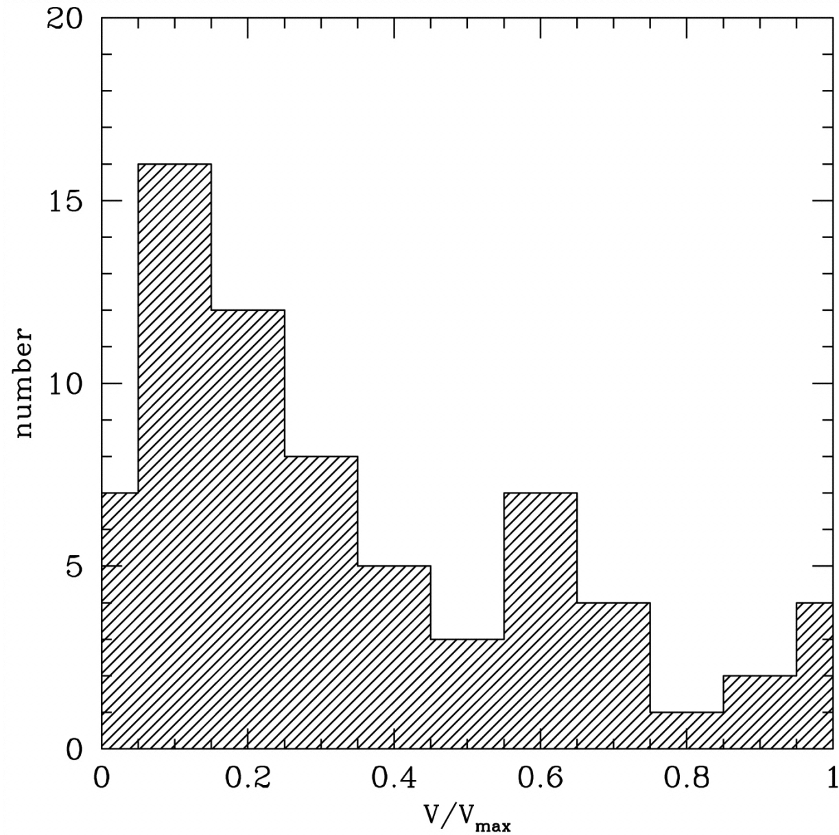
Fig. 21. from The Evolution of EarlyType Field Galaxies Selected from a NICMOS Map of the Hubble Deep Field North Stanford et al. 2004 AJ 127 131 doi:10.1086/380612 https://dx.doi.org/10.1086/380612 © 2004. The American Astronomical Society. All rights reserved. Printed in U.S.A.
