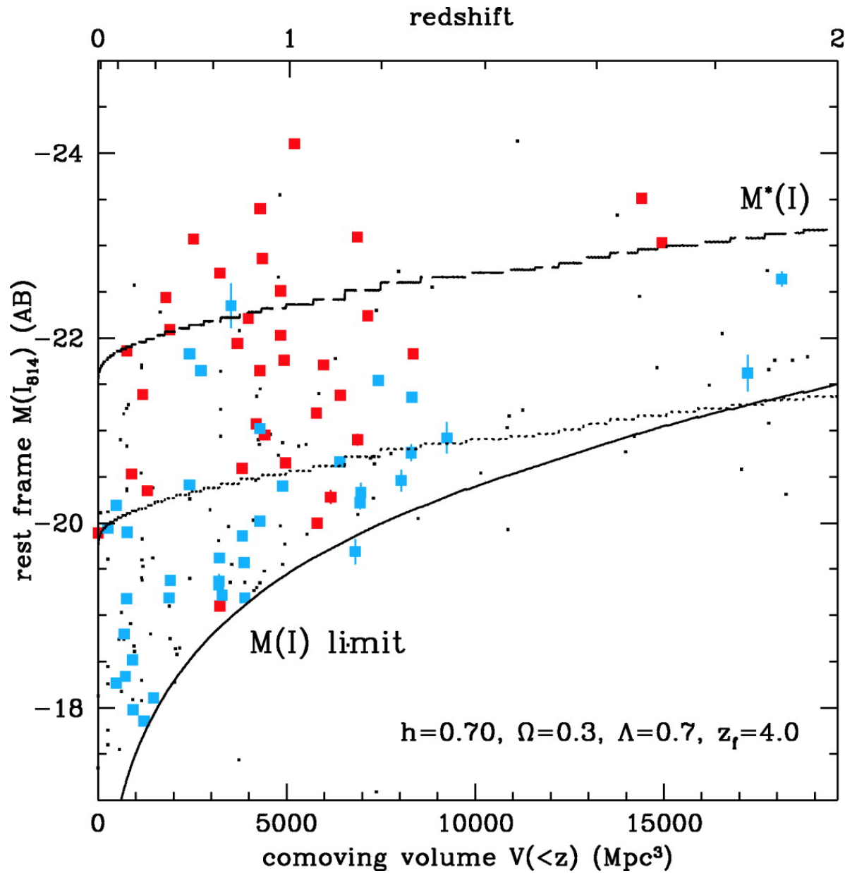
Fig. 18. from The Evolution of EarlyType Field Galaxies Selected from a NICMOS Map of the Hubble Deep Field North Stanford et al. 2004 AJ 127 131 doi:10.1086/380612 https://dx.doi.org/10.1086/380612
