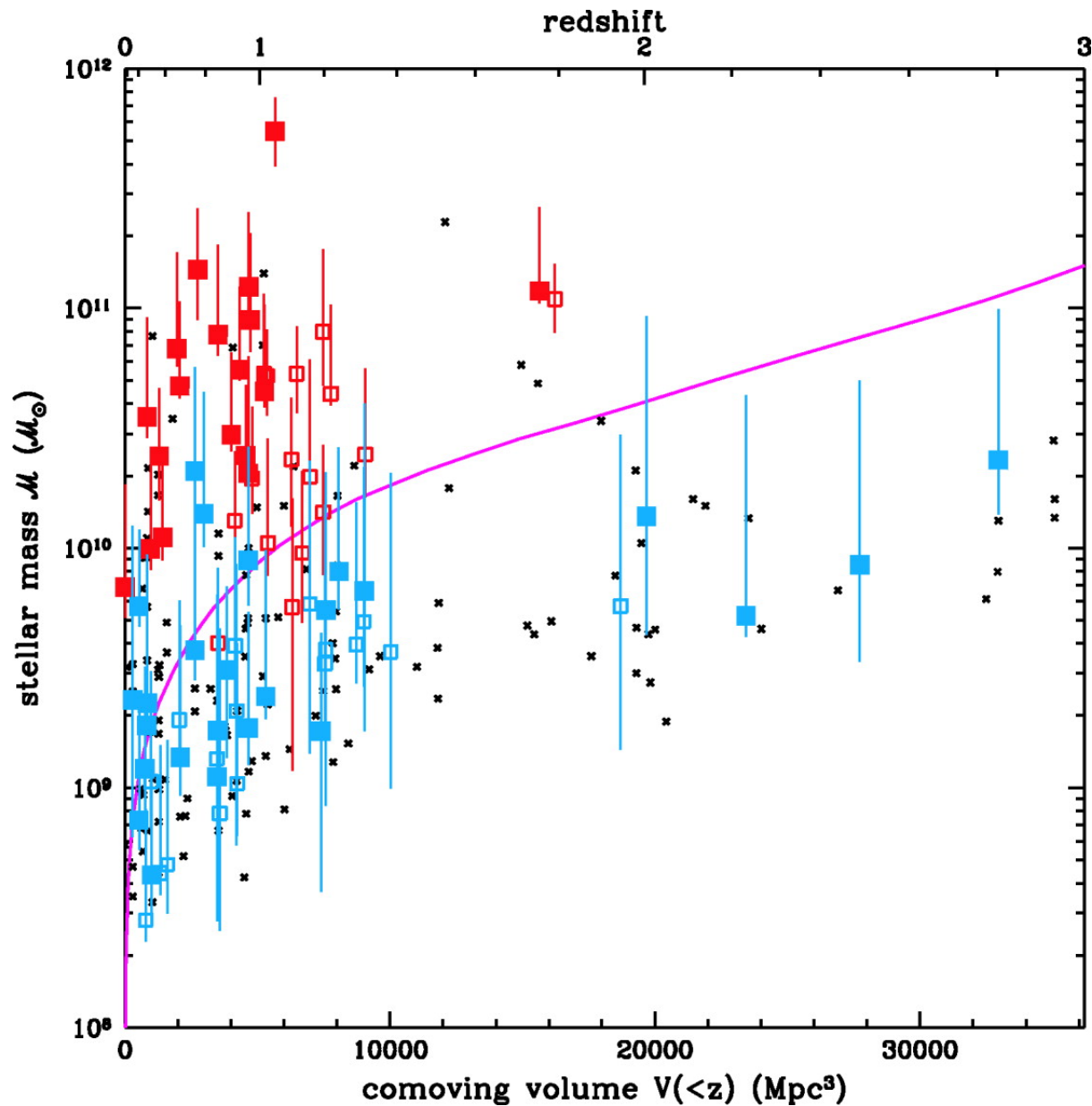
Fig. 15. from The Evolution of EarlyType Field Galaxies Selected from a NICMOS Map of the Hubble Deep Field North Stanford et al. 2004 AJ 127 131 doi:10.1086/380612 https://dx.doi.org/10.1086/380612 © 2004. The American Astronomical Society. All rights reserved. Printed in U.S.A.
