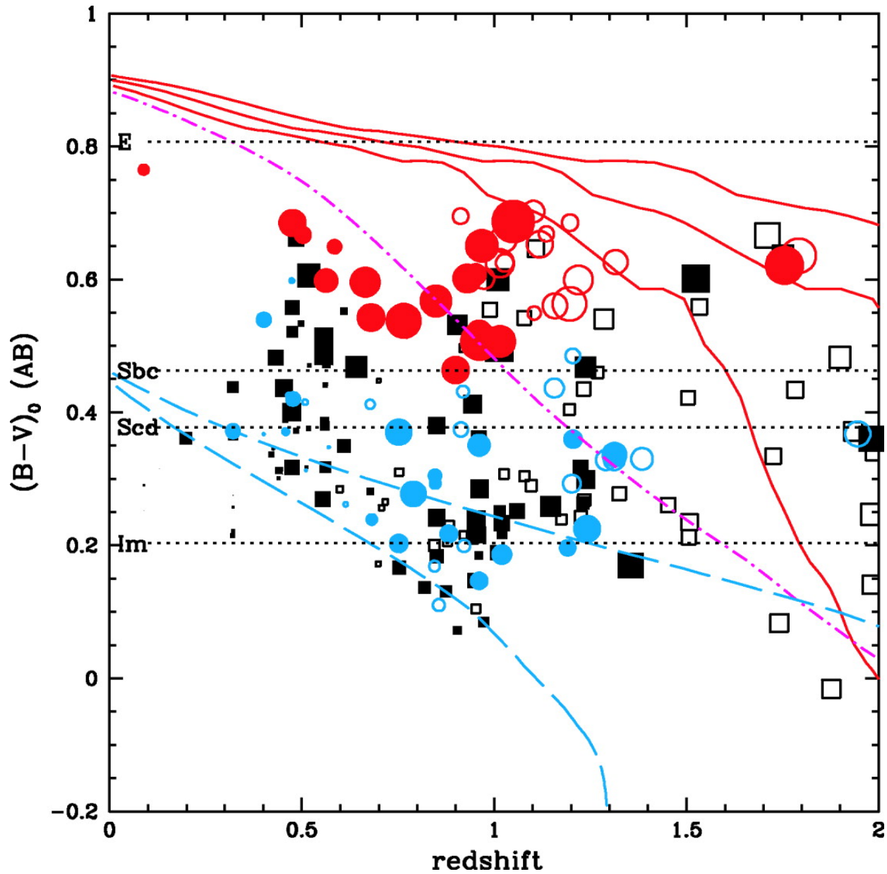
Fig. 13. from The Evolution of EarlyType Field Galaxies Selected from a NICMOS Map of the Hubble Deep Field North Stanford et al. 2004 AJ 127 131 doi:10.1086/380612 https://dx.doi.org/10.1086/380612
