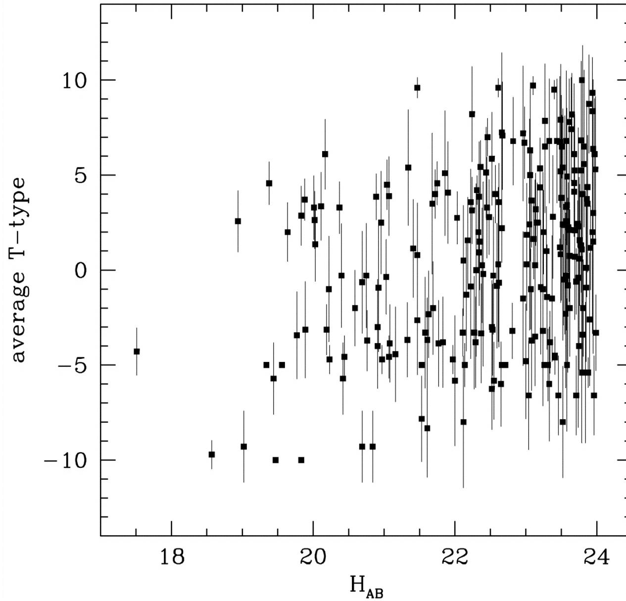
Fig. 1. from The Evolution of EarlyType Field Galaxies Selected from a NICMOS Map of the Hubble Deep Field North Stanford et al. 2004 AJ 127 131 doi:10.1086/380612 https://dx.doi.org/10.1086/380612 © 2004. The American Astronomical Society. All rights reserved. Printed in U.S.A.
