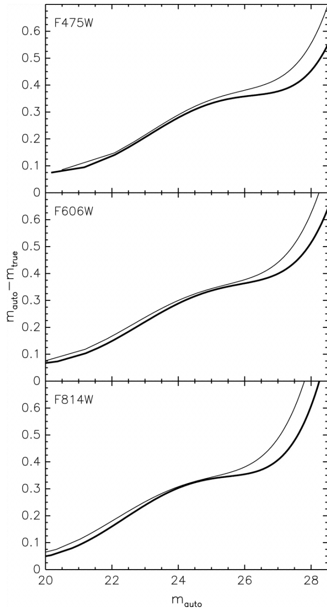
Fig. 9. from Faint Galaxies in Deep Advanced Camera for Surveys Observations Benítez et al. 2004 ApJS 150 1 doi:10.1086/380120 https://dx.doi.org/10.1086/380120 © 2004. The American Astronomical Society. All rights reserved. Printed in U.S.A.
