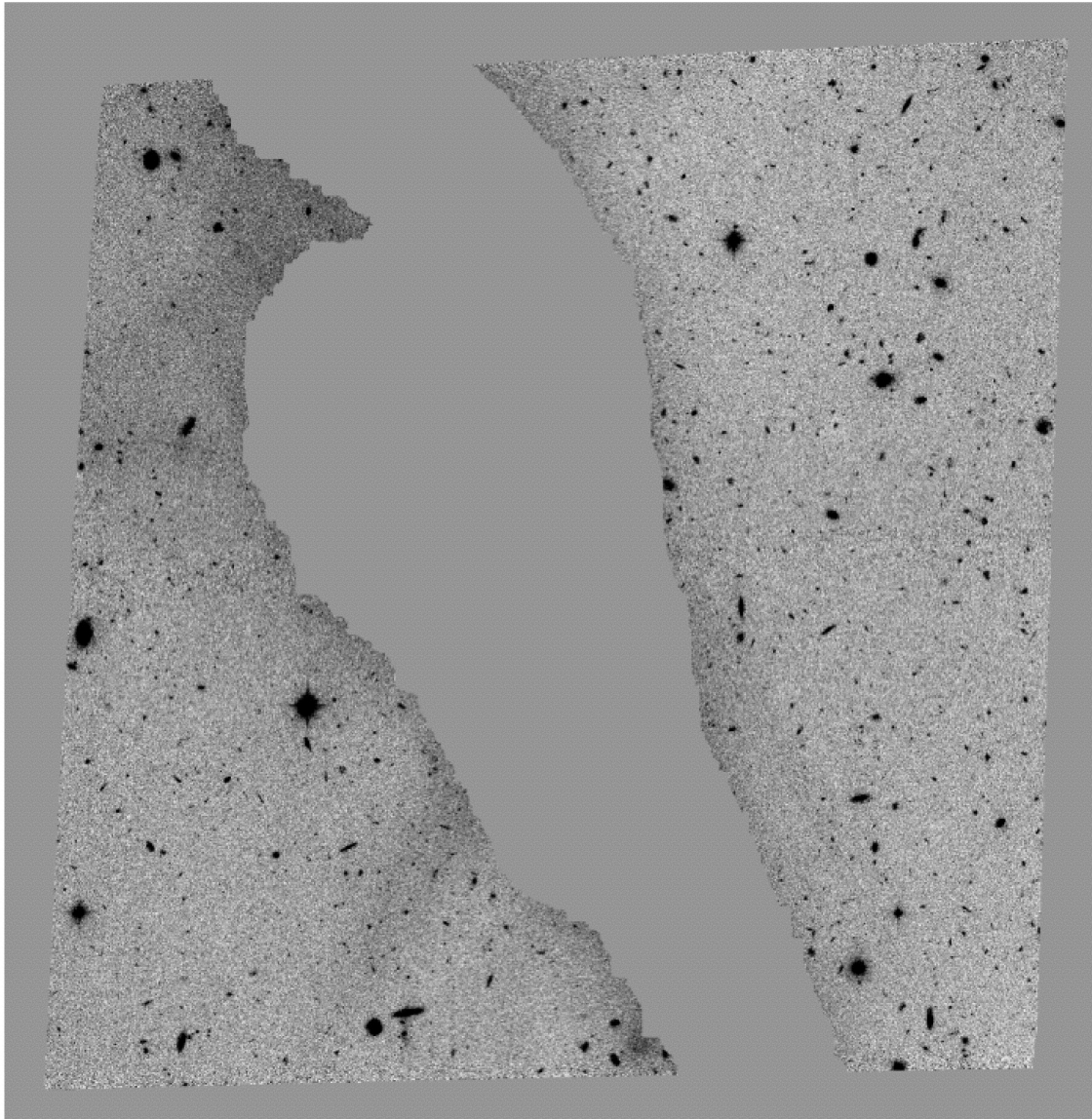
Fig. 7. from Faint Galaxies in Deep Advanced Camera for Surveys Observations Benítez et al. 2004 ApJS 150 1 doi:10.1086/380120 https://dx.doi.org/10.1086/380120 © 2004. The American Astronomical Society. All rights reserved. Printed in U.S.A.
