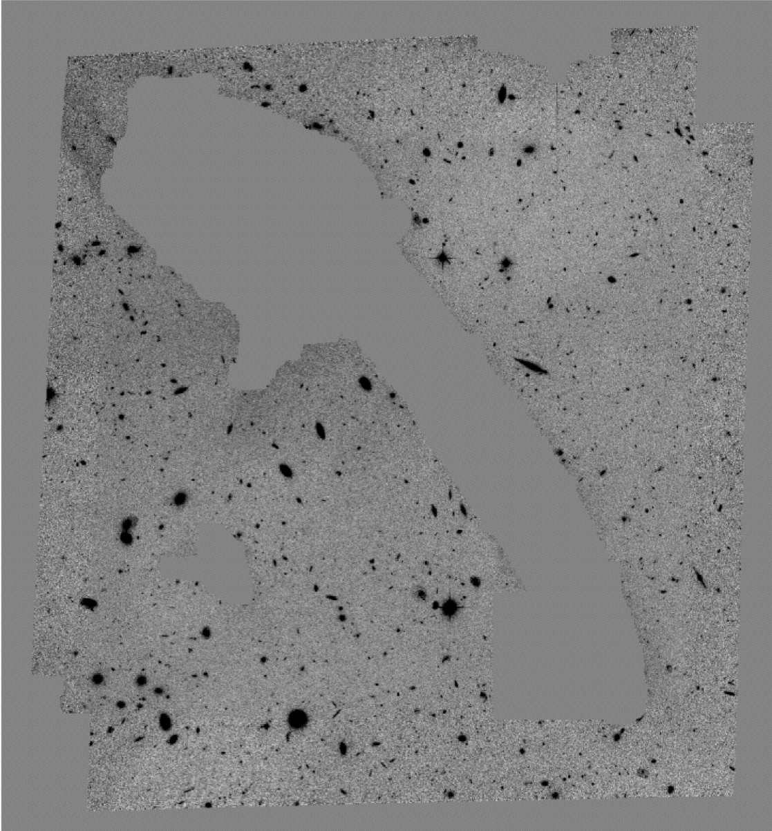
Fig. 6. from Faint Galaxies in Deep Advanced Camera for Surveys Observations Benítez et al. 2004 ApJS 150 1 doi:10.1086/380120 https://dx.doi.org/10.1086/380120 © 2004. The American Astronomical Society. All rights reserved. Printed in U.S.A.
