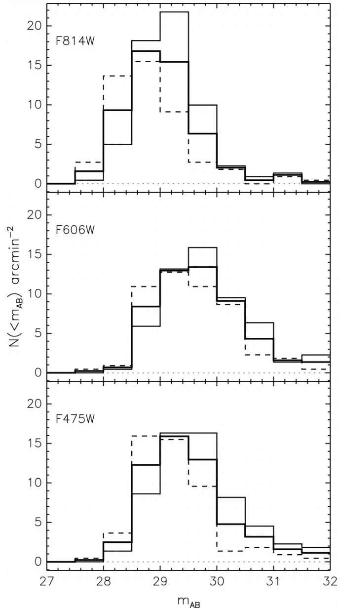
Fig. 5. from Faint Galaxies in Deep Advanced Camera for Surveys Observations Benítez et al. 2004 ApJS 150 1 doi:10.1086/380120 https://dx.doi.org/10.1086/380120 © 2004. The American Astronomical Society. All rights reserved. Printed in U.S.A.
