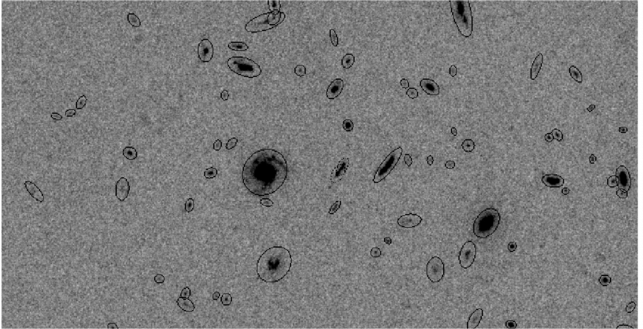
Fig. 4. from Faint Galaxies in Deep Advanced Camera for Surveys Observations Benítez et al. 2004 ApJS 150 1 doi:10.1086/380120 https://dx.doi.org/10.1086/380120 © 2004. The American Astronomical Society. All rights reserved. Printed in U.S.A.
