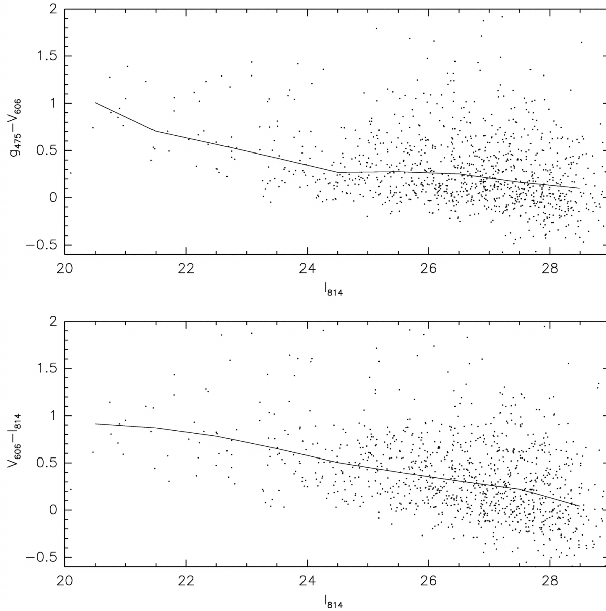
Fig. 20. from Faint Galaxies in Deep Advanced Camera for Surveys Observations Benítez et al. 2004 ApJS 150 1 doi:10.1086/380120 https://dx.doi.org/10.1086/380120 © 2004. The American Astronomical Society. All rights reserved. Printed in U.S.A.
