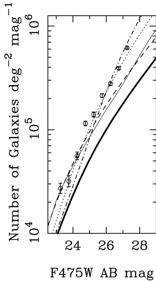
Fig. 19. from Faint Galaxies in Deep Advanced Camera for Surveys Observations Benítez et al. 2004 ApJS 150 1 doi:10.1086/380120 https://dx.doi.org/10.1086/380120 © 2004. The American Astronomical Society. All rights reserved. Printed in U.S.A.
