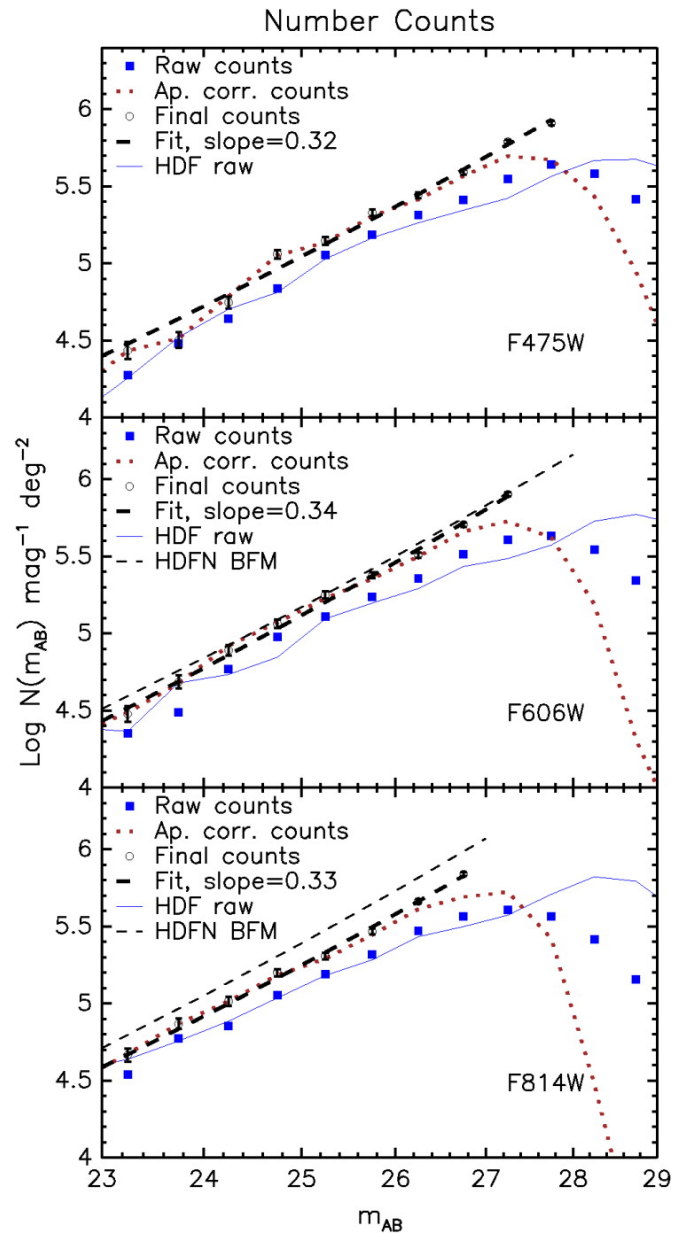
Fig. 18. from Faint Galaxies in Deep Advanced Camera for Surveys Observations Benítez et al. 2004 ApJS 150 1 doi:10.1086/380120 https://dx.doi.org/10.1086/380120 © 2004. The American Astronomical Society. All rights reserved. Printed in U.S.A.
