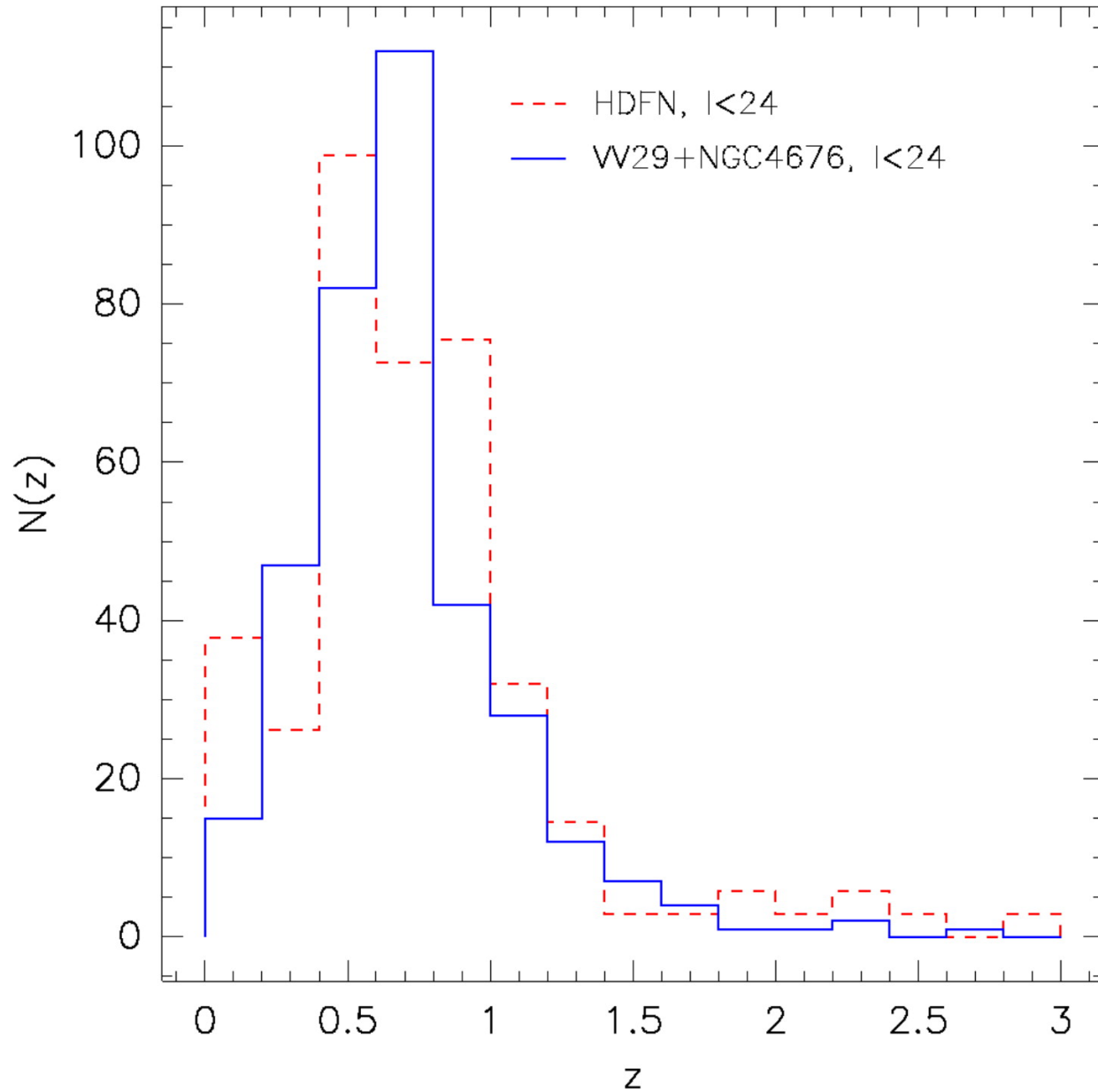
Fig. 17. from Faint Galaxies in Deep Advanced Camera for Surveys Observations Benítez et al. 2004 ApJS 150 1 doi:10.1086/380120 https://dx.doi.org/10.1086/380120 © 2004. The American Astronomical Society. All rights reserved. Printed in U.S.A.
