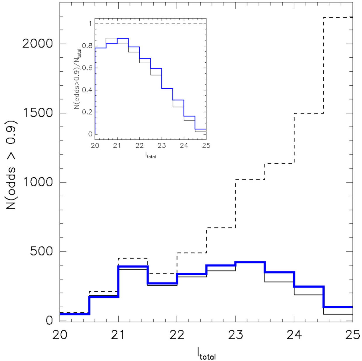
Fig. 15. from Faint Galaxies in Deep Advanced Camera for Surveys Observations Benítez et al. 2004 ApJS 150 1 doi:10.1086/380120 https://dx.doi.org/10.1086/380120 © 2004. The American Astronomical Society. All rights reserved. Printed in U.S.A.
