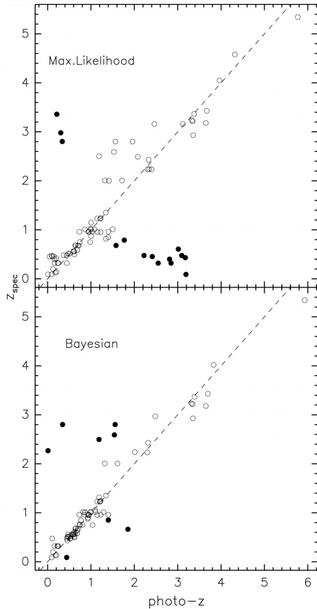
Fig. 14. from Faint Galaxies in Deep Advanced Camera for Surveys Observations Benítez et al. 2004 ApJS 150 1 doi:10.1086/380120 https://dx.doi.org/10.1086/380120 © 2004. The American Astronomical Society. All rights reserved. Printed in U.S.A.
