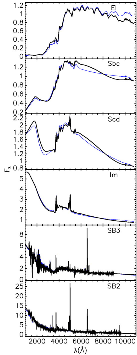
Fig. 13. from Faint Galaxies in Deep Advanced Camera for Surveys Observations Benítez et al. 2004 ApJS 150 1 doi:10.1086/380120 https://dx.doi.org/10.1086/380120
