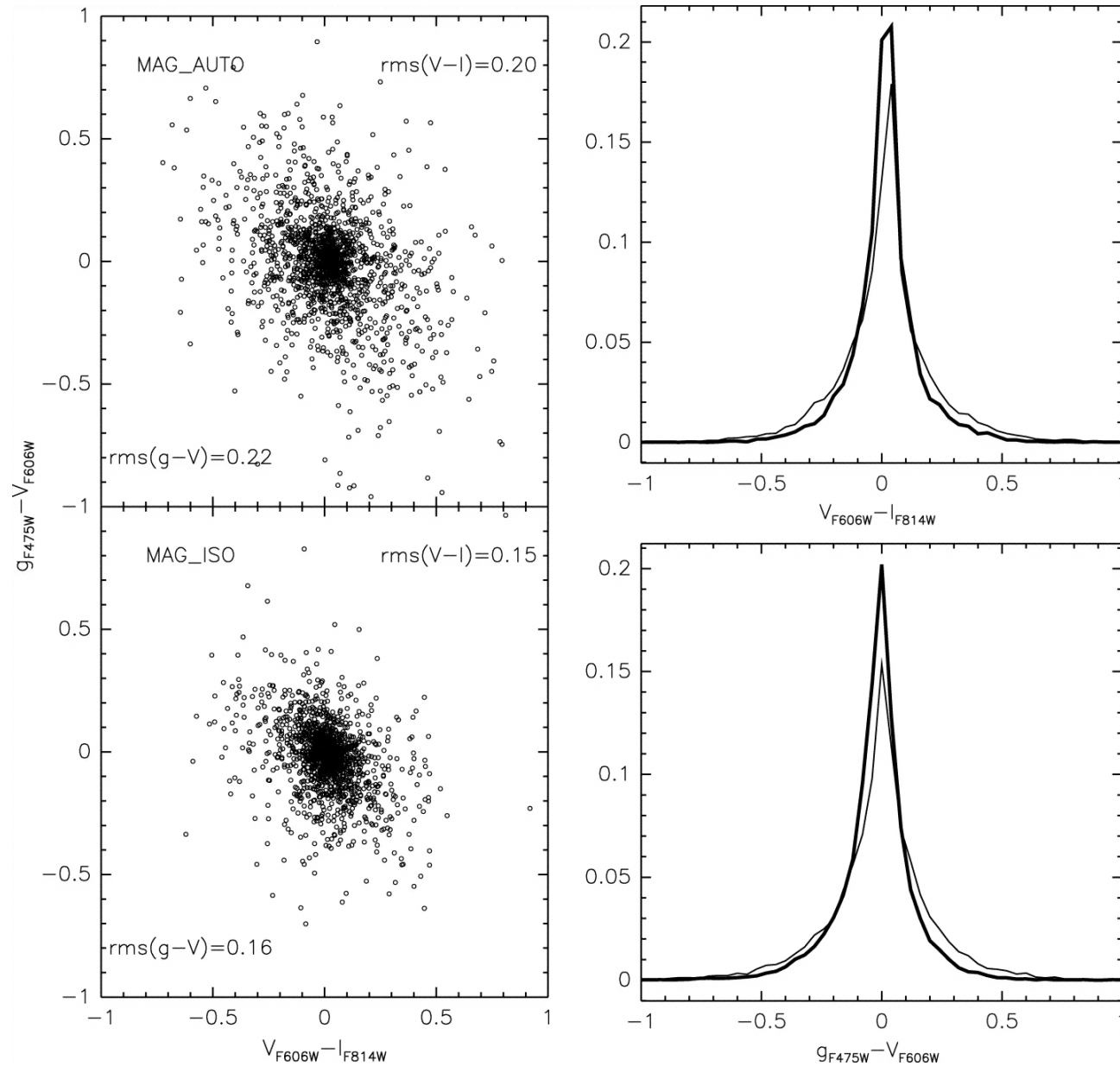
Fig. 10. from Faint Galaxies in Deep Advanced Camera for Surveys Observations Benítez et al. 2004 ApJS 150 1 doi:10.1086/380120 https://dx.doi.org/10.1086/380120 © 2004. The American Astronomical Society. All rights reserved. Printed in U.S.A.
