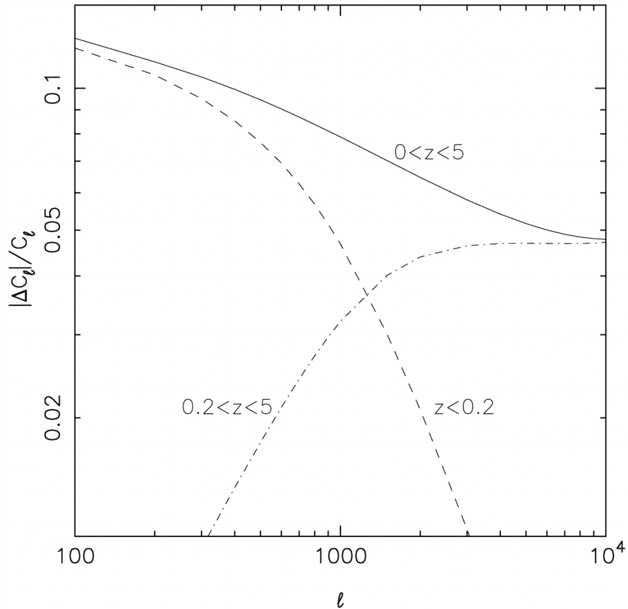
Fig. 3. from Contamination of Cluster Radio Sources in the Measurement of the Thermal SunyaevZel'dovich Angular Power Spectrum Zhou & Wu 2004 ApJ 600 501 doi:10.1086/380119 https://dx.doi.org/10.1086/380119 © 2004. The American Astronomical Society. All rights reserved. Printed in U.S.A.
