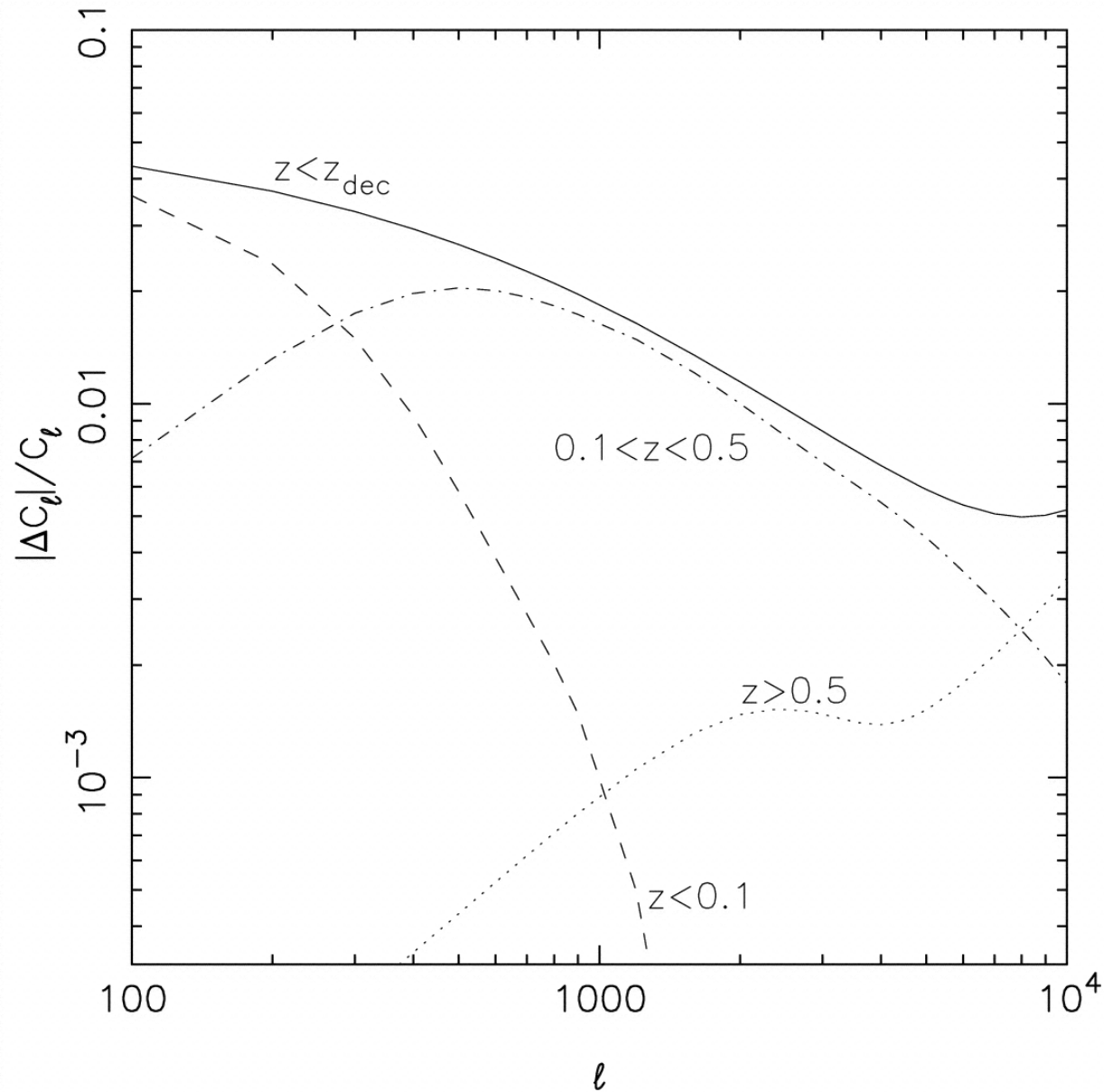
Fig. 1. from Contamination of Cluster Radio Sources in the Measurement of the Thermal SunyaevZel'dovich Angular Power Spectrum Zhou & Wu 2004 ApJ 600 501 doi:10.1086/380119 https://dx.doi.org/10.1086/380119 © 2004. The American Astronomical Society. All rights reserved. Printed in U.S.A.
