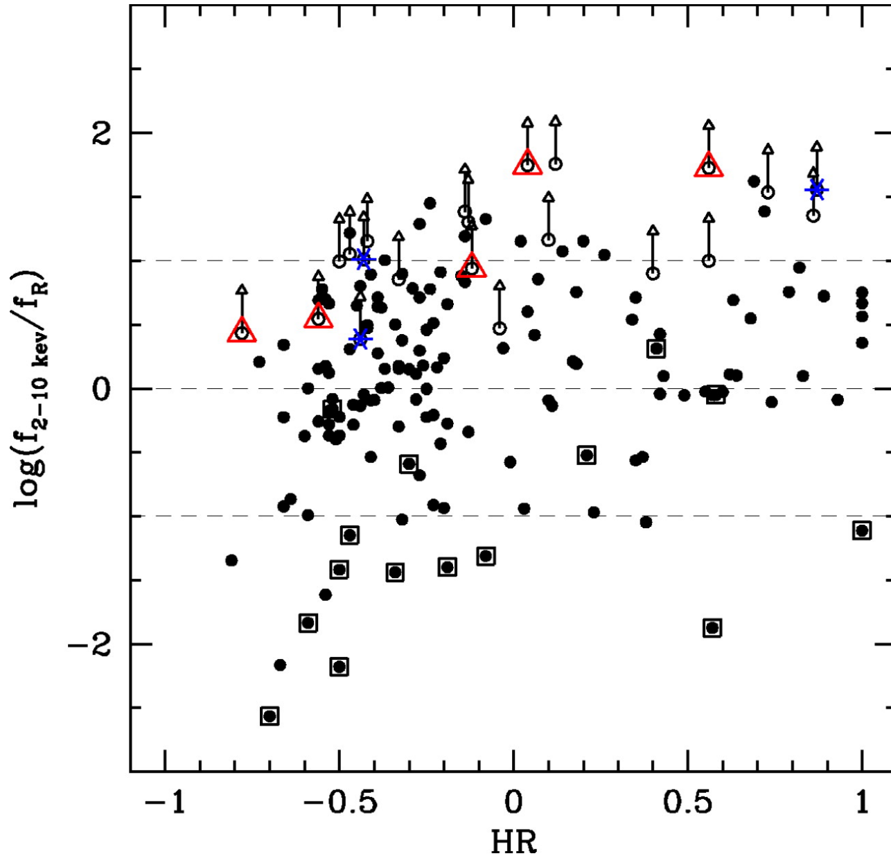
Fig. 9. from The 172 ks Chandra Exposure of the LALA Bootes Field: XRay Source Catalog Wang et al. 2004 AJ 127 213 doi:10.1086/379960 https://dx.doi.org/10.1086/379960 © 2004. The American Astronomical Society. All rights reserved. Printed in U.S.A.
