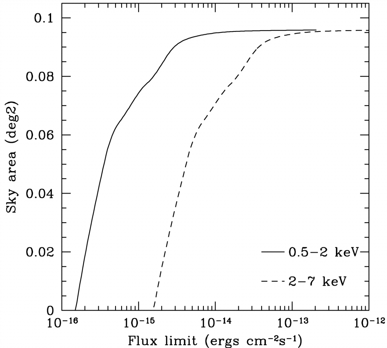
Fig. 5. from The 172 ks Chandra Exposure of the LALA Bootes Field: XRay Source Catalog Wang et al. 2004 AJ 127 213 doi:10.1086/379960 https://dx.doi.org/10.1086/379960 © 2004. The American Astronomical Society. All rights reserved. Printed in U.S.A.
