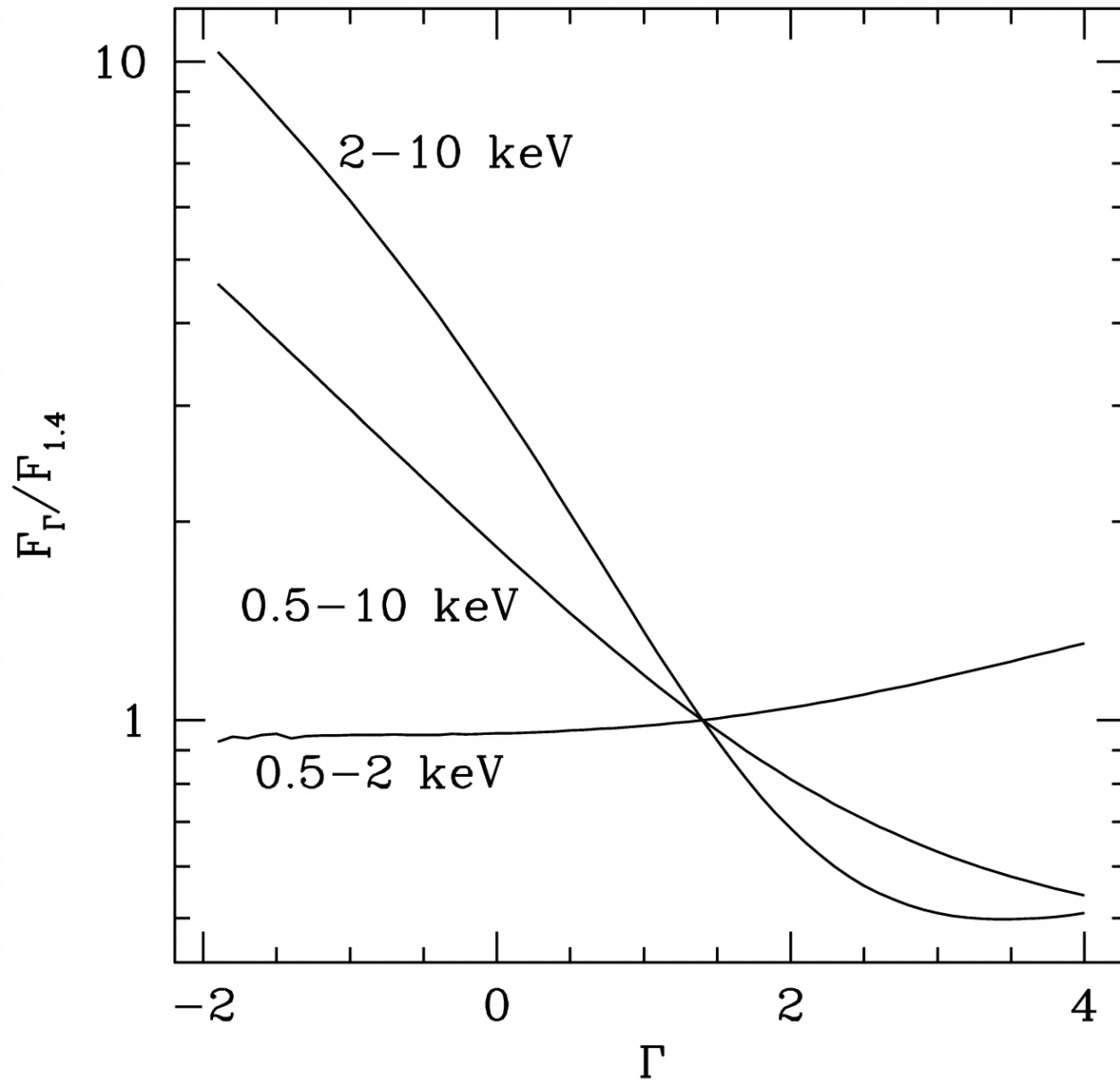
Fig. 3. from The 172 ks Chandra Exposure of the LALA Bootes Field: XRay Source Catalog Wang et al. 2004 AJ 127 213 doi:10.1086/379960 https://dx.doi.org/10.1086/379960 © 2004. The American Astronomical Society. All rights reserved. Printed in U.S.A.
