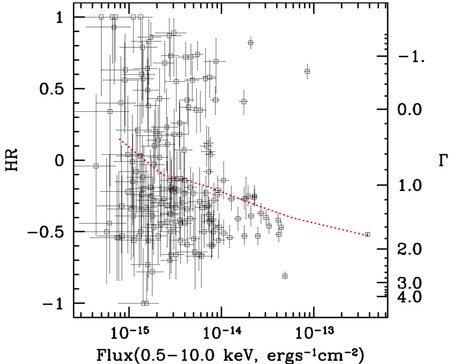
Fig. 2. from The 172 ks Chandra Exposure of the LALA Bootes Field: XRay Source Catalog Wang et al. 2004 AJ 127 213 doi:10.1086/379960 https://dx.doi.org/10.1086/379960 © 2004. The American Astronomical Society. All rights reserved. Printed in U.S.A.
