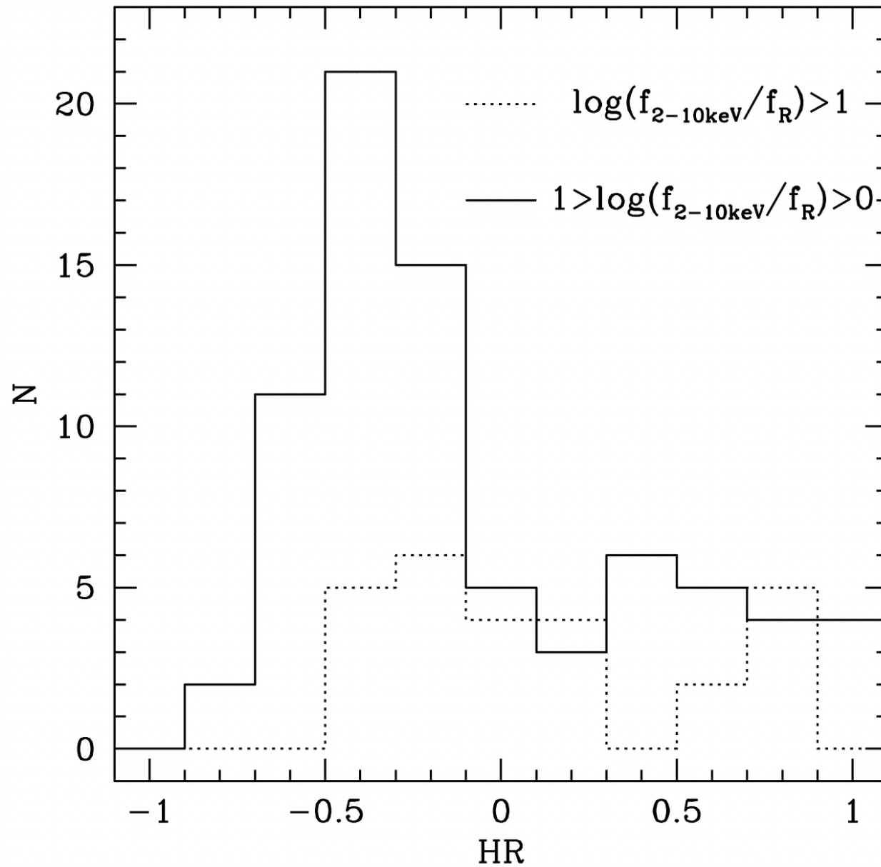
Fig. 10. from The 172 ks Chandra Exposure of the LALA Bootes Field: XRay Source Catalog Wang et al. 2004 AJ 127 213 doi:10.1086/379960 https://dx.doi.org/10.1086/379960 © 2004. The American Astronomical Society. All rights reserved. Printed in U.S.A.
