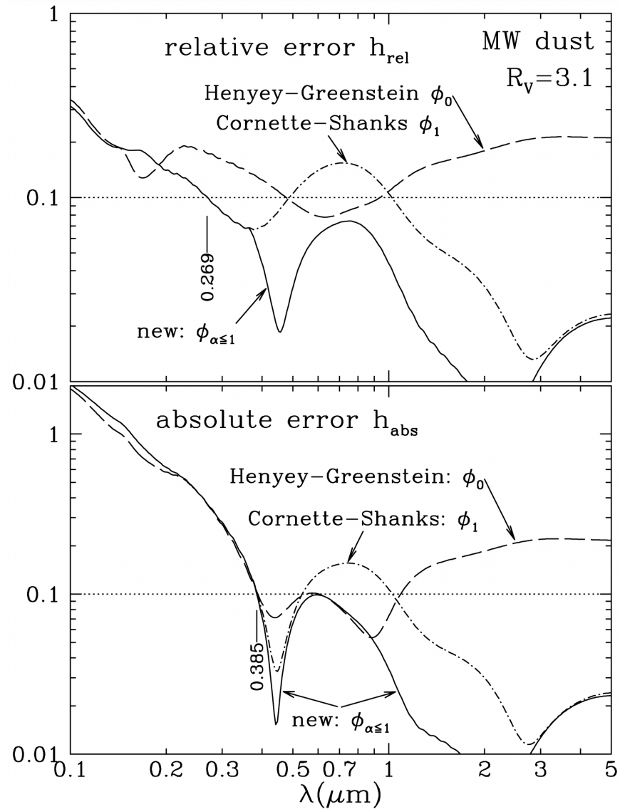
Fig. 8. from Scattering by Interstellar Dust Grains. I. Optical and Ultraviolet Draine 2003 ApJ 598 1017 doi:10.1086/379118 https://dx.doi.org/10.1086/379118 © 2003. The American Astronomical Society. All rights reserved. Printed in U.S.A.
