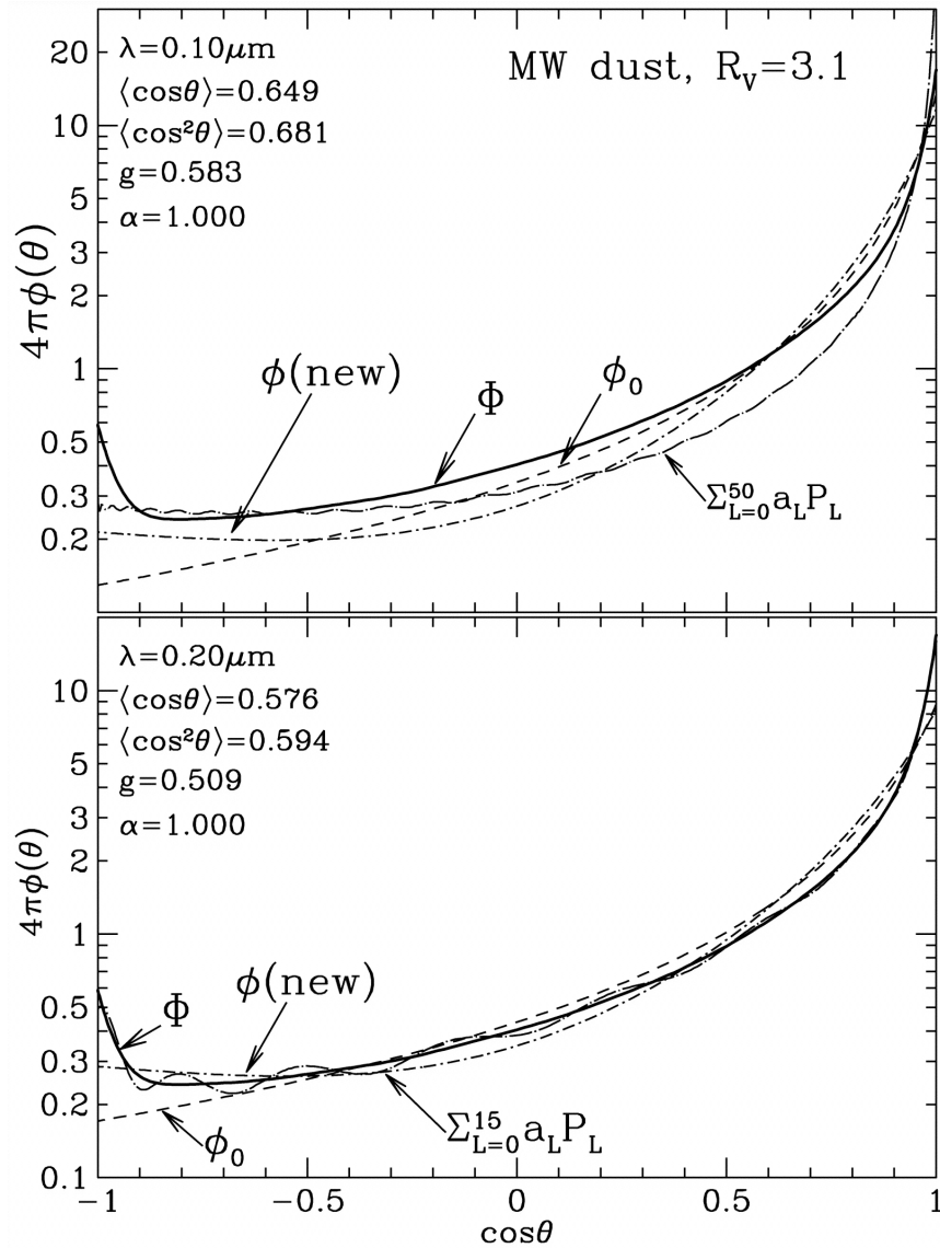
Fig. 7. from Scattering by Interstellar Dust Grains. I. Optical and Ultraviolet Draine 2003 ApJ 598 1017 doi:10.1086/379118 https://dx.doi.org/10.1086/379118 © 2003. The American Astronomical Society. All rights reserved. Printed in U.S.A.
